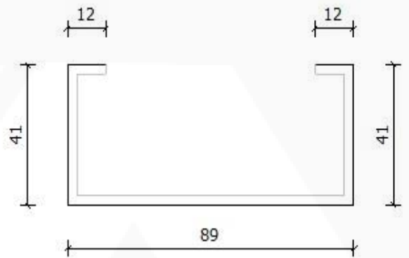
• S550GD / Z275 / BMT: 1.15 mm
