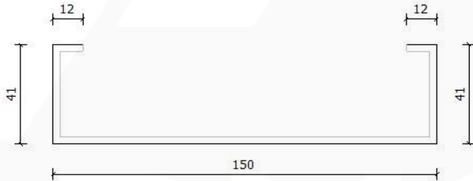
• S550GD / Z275 / BMT: 1.15 mm
