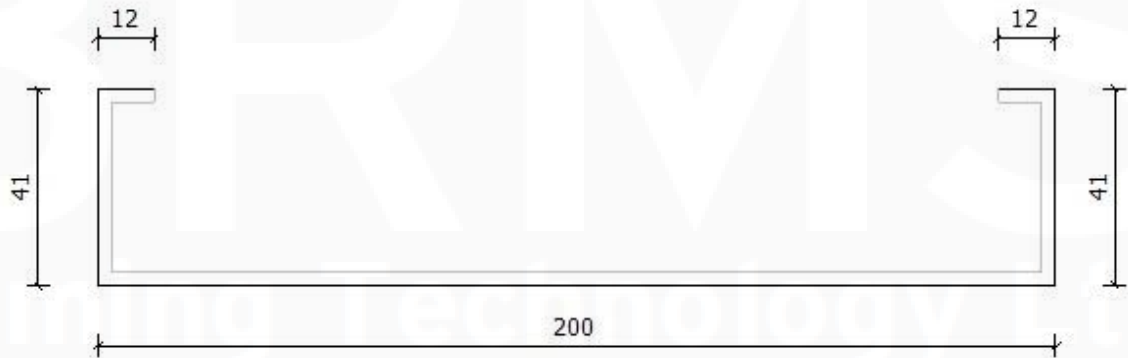
• S550GD / Z275 / BMT: 1.15 mm
